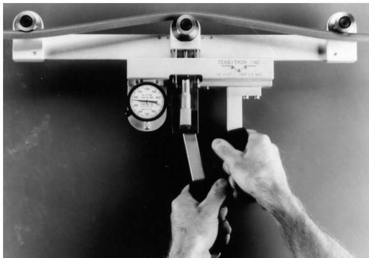
( For instrument ranges 500 lb and lower, the instrument width is 16.75" ) ( For the 1000 lb range, the instrument width is 19.75" )
